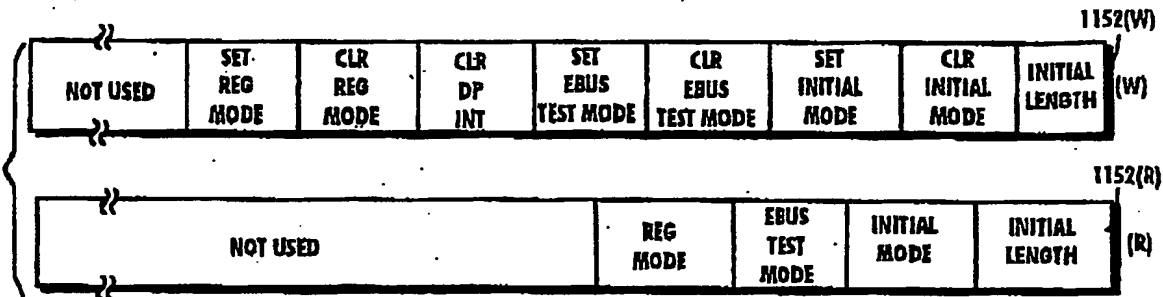
Fig. 39A CPU STATUS/CONTROL REGISTER (R/W)
